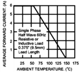
FIG.2- MAXIMUM FORWARD CURRENT DERATING CURVE
