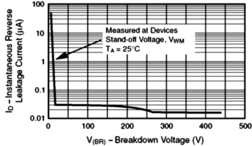
Fig. 7 – Typical Reverse Leakage Characteristics
