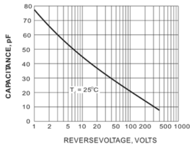
Fig.5-TYPICAL JUNCTION CAPACITANCE
