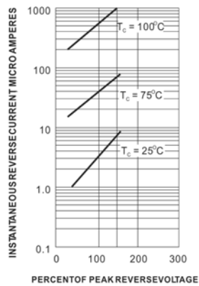
Fig.3-TYPICAL REVERSE CHARACTERISTIC
